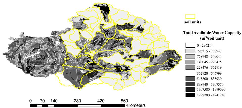
Fig. 2. Available soil water content in 2 m depth soil layer (Yellow lines indicate sub basin of Tisza River)
